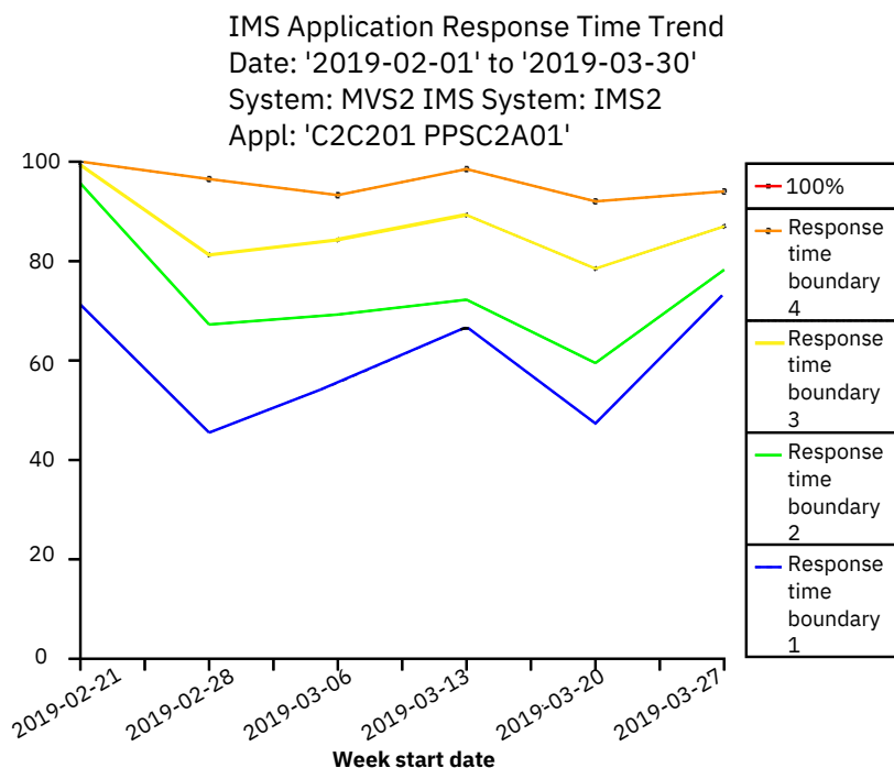
Figure 18. Graphic reports example
