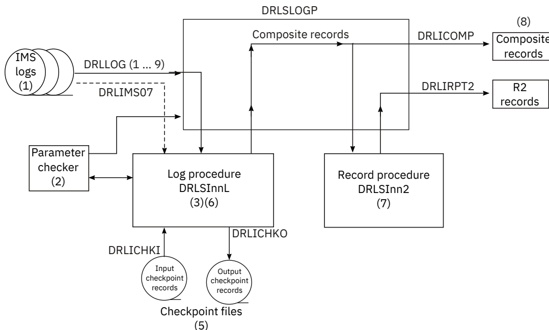
Figure 10. Data flow through DRLSLOGP
