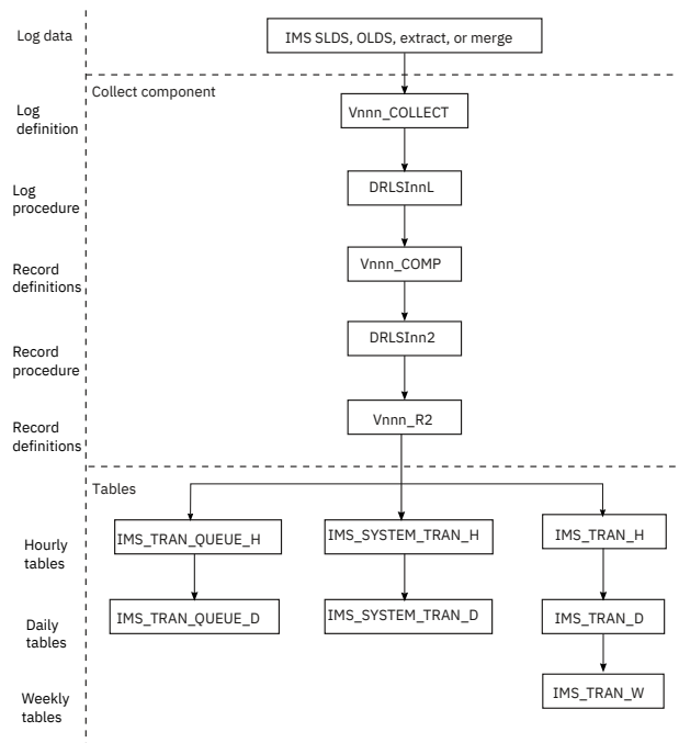
Figure 13. Data flow: Transaction Transit Time subcomponent
