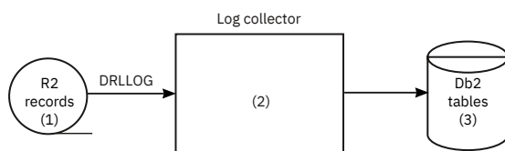
Figure 11. Data flow through IMS CSQ light feature
