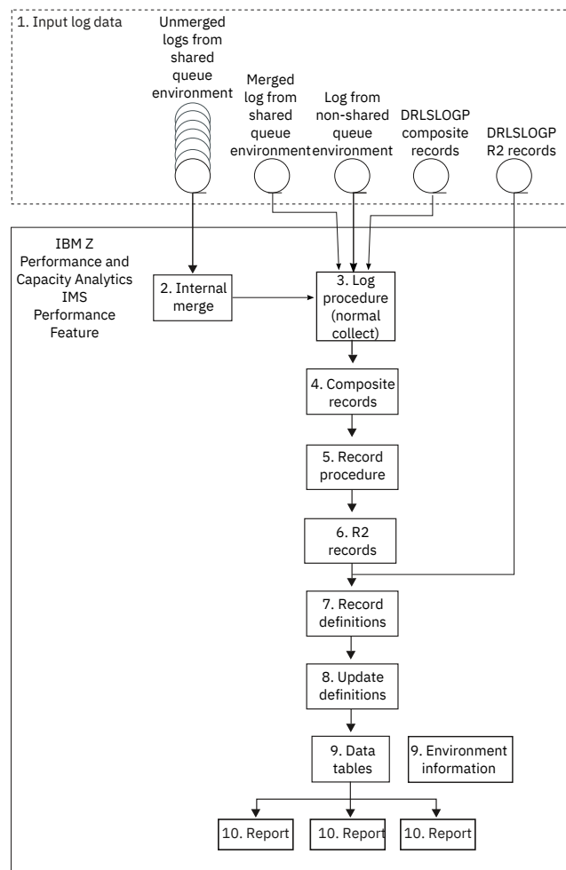
Figure 2. Overview of data collection using the IMS Performance Feature
