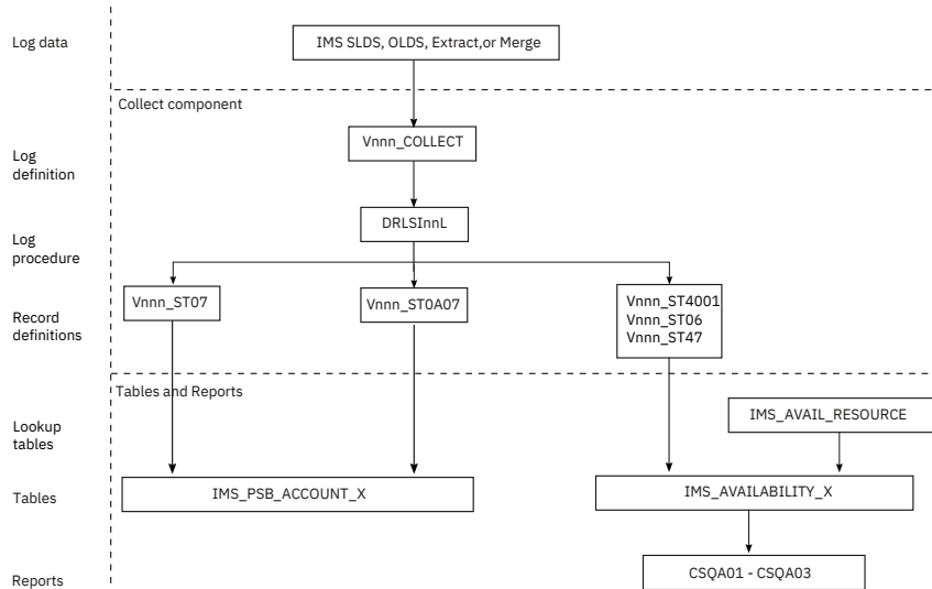
Figure 12. Data flow: Account and Availability subcomponent
